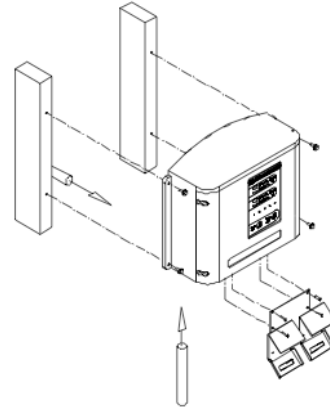
Figure 6. Wall mounting of 60 amp
