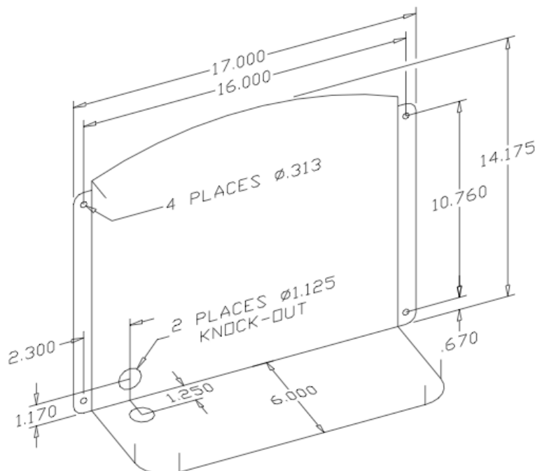
Figure 7. 60 amp Charger Installation Template
