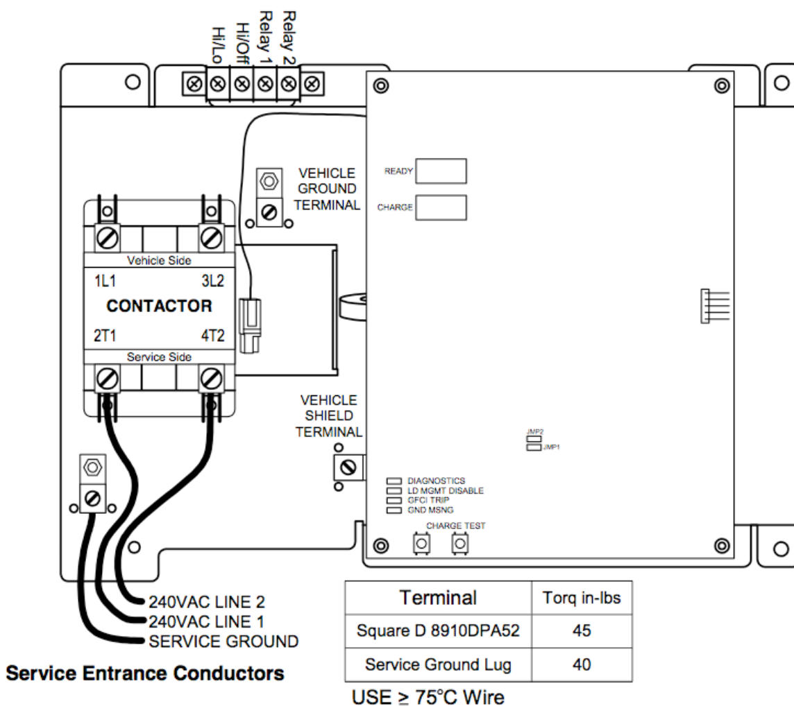
Figure 8. 60 amp Charger Service Wiring
